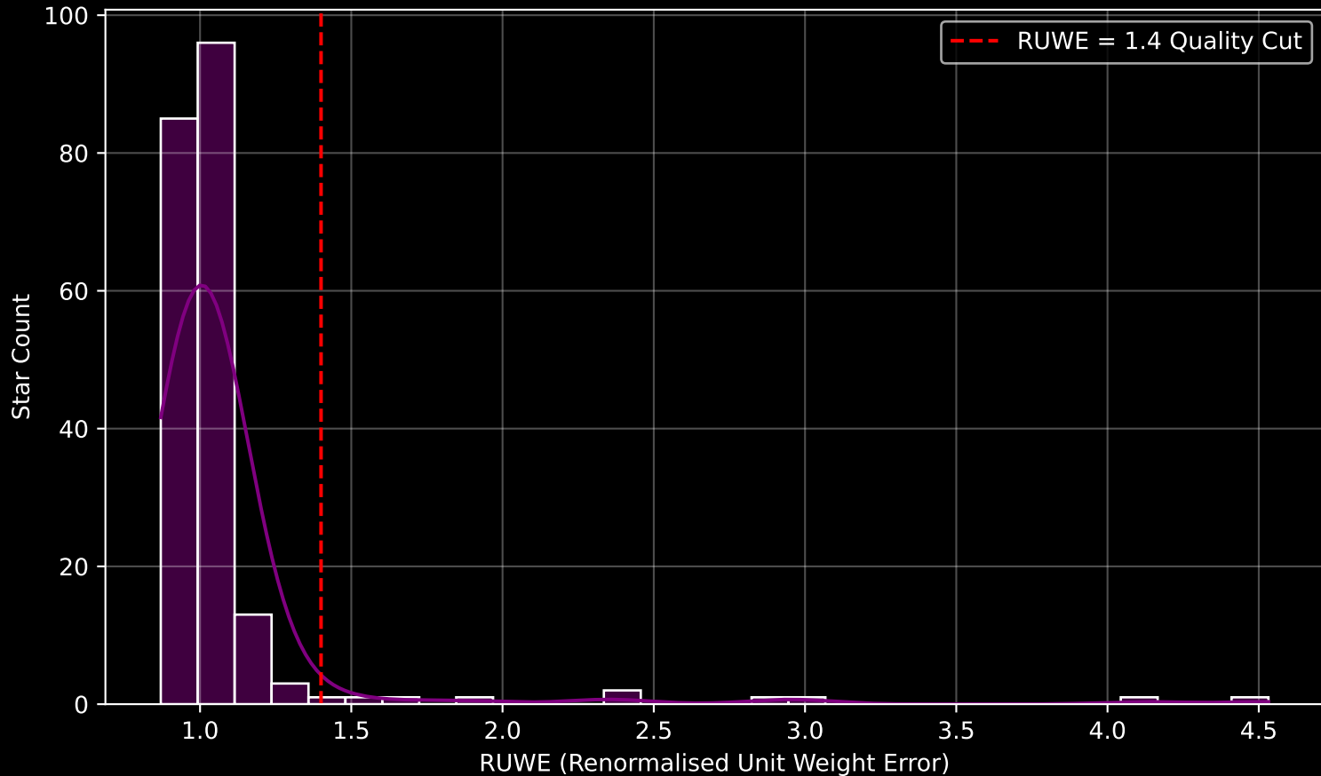
GAPOGEE DR17 Field [340+00] RUWE Distribution (n= 207)
