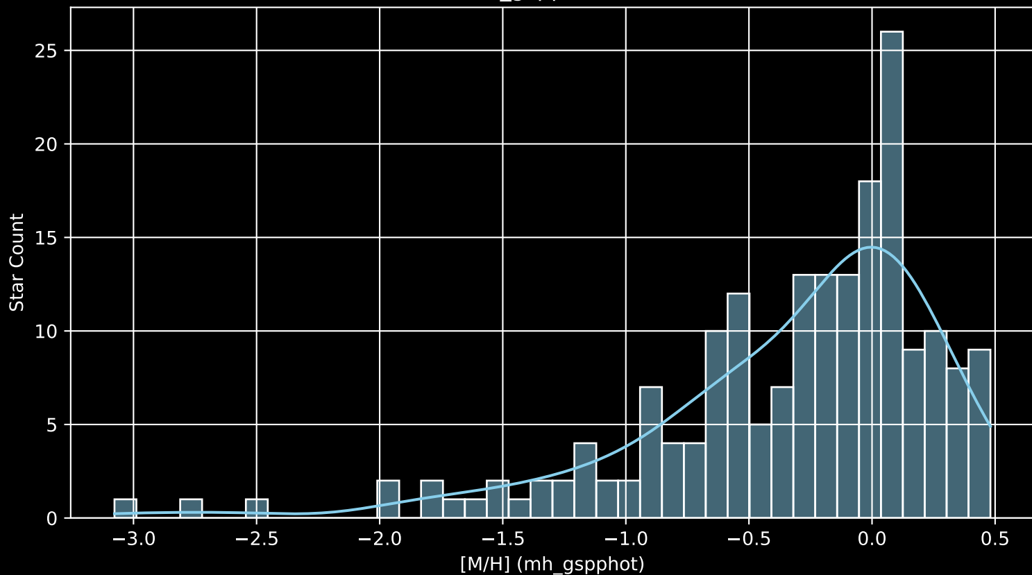
APOGEE DR17 Field: [340+00 [M/H] (mh_gspphot) (n= 192)
