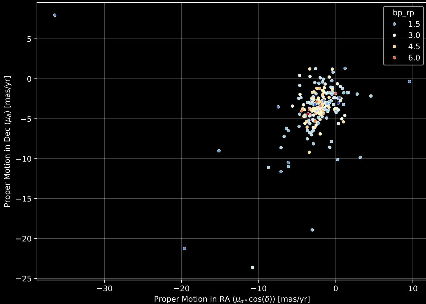
APOGEE DR17 Field: [340+00] Proper Motion Diagram (n= 209)
