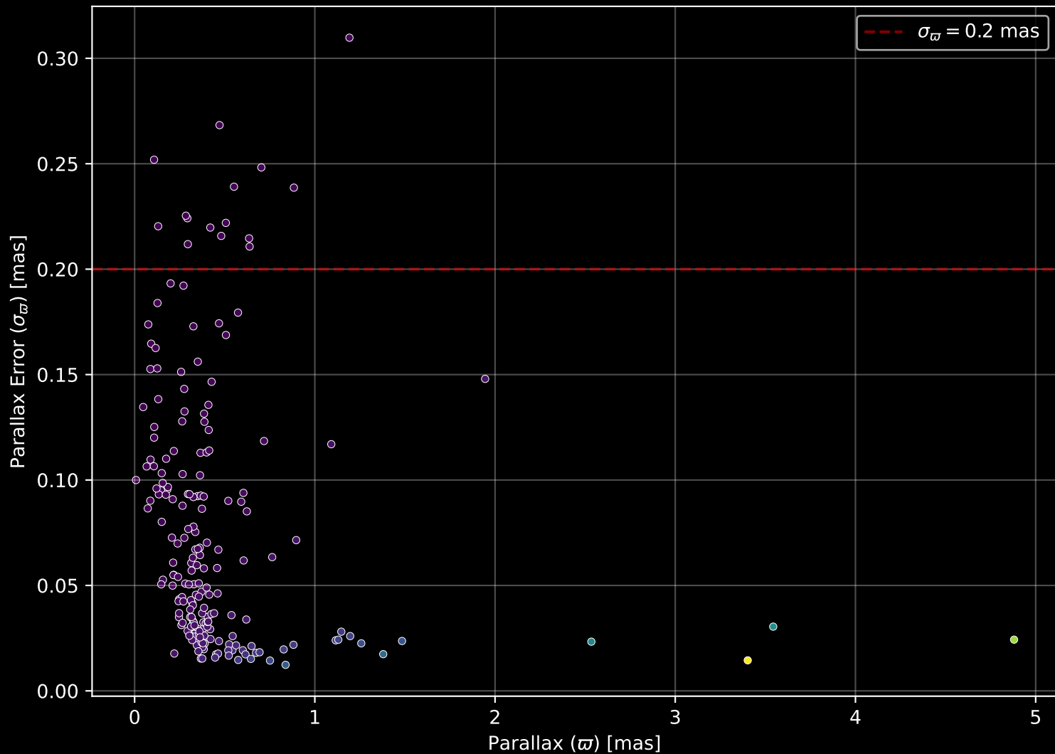
APOGEE DR17 Field: [340+00] Parallax Quality (n= 209)
