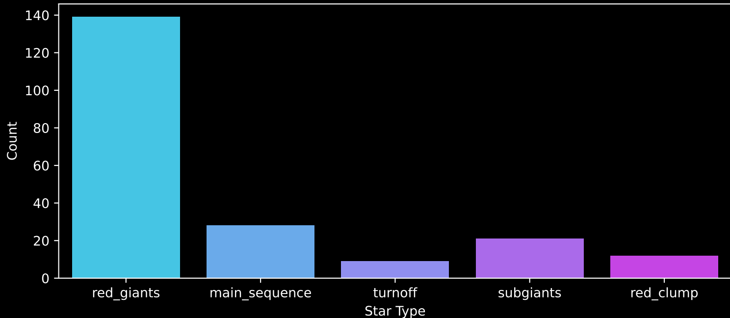
APOGEE DR17 Field: [340+00] Count plot of Star Type
