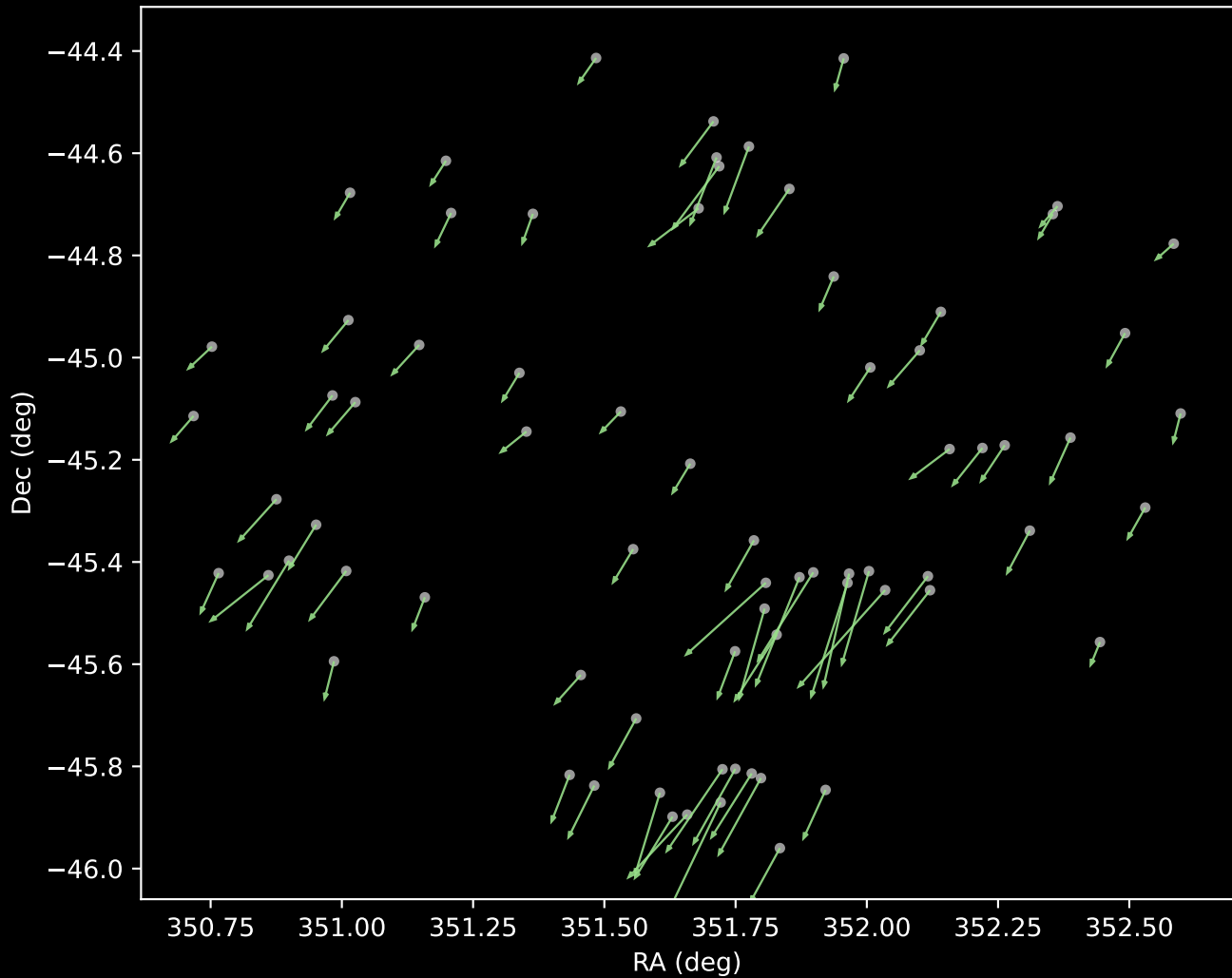
APOGEE DR17 Cluster 5 Proper Motion Vectors (n=74)
